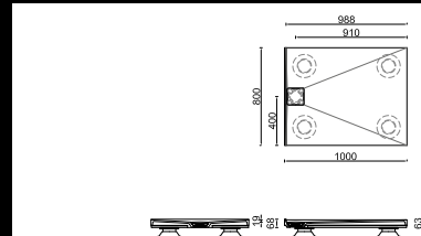
DW-RA-80-100: 800 x 1000 MM
