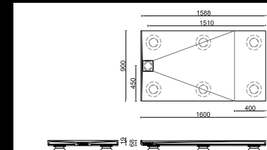
DW-RA-90-160: 900 x 1600 mm
