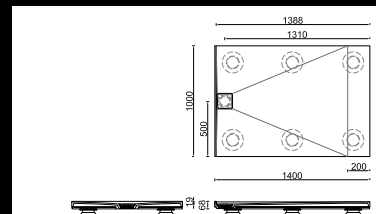
DW-RA-100-140: 1000 x 1400 mm
