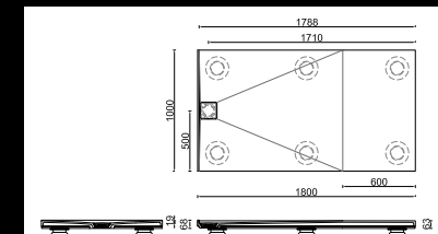
DW-RA-100-180: 1000 x 1800 mm
