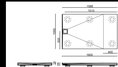
DW-RA-100-160: 1000 x 1600 MM
