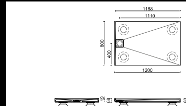
DW-RA-80-120: 800 x 1200 MM
