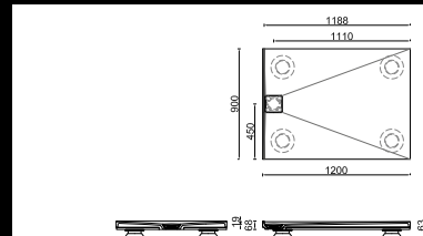
DW-RA-90-120: 900 x 1200 mm
